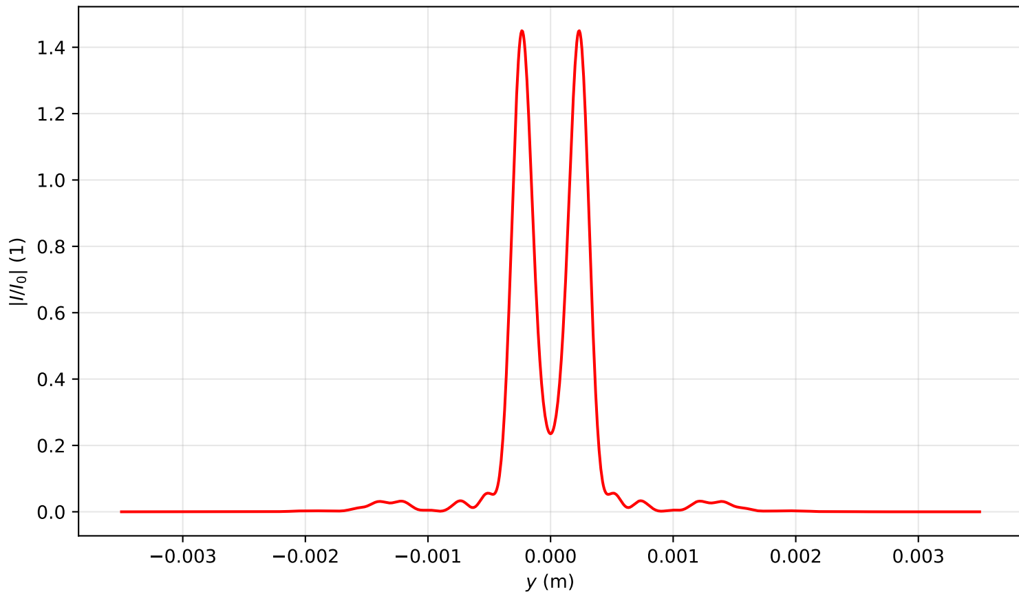
Intensity profile I(x=0, y, z=1.911)/I_0 , P_{in}=3.0P_{cr} , artificial time
